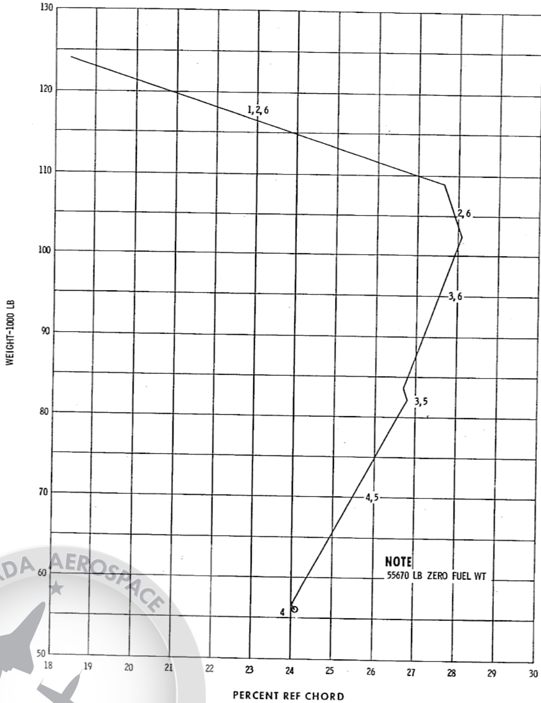
TYPICAL C. G. TRAVEL 2400 LB AFT TRANSFER STOP
