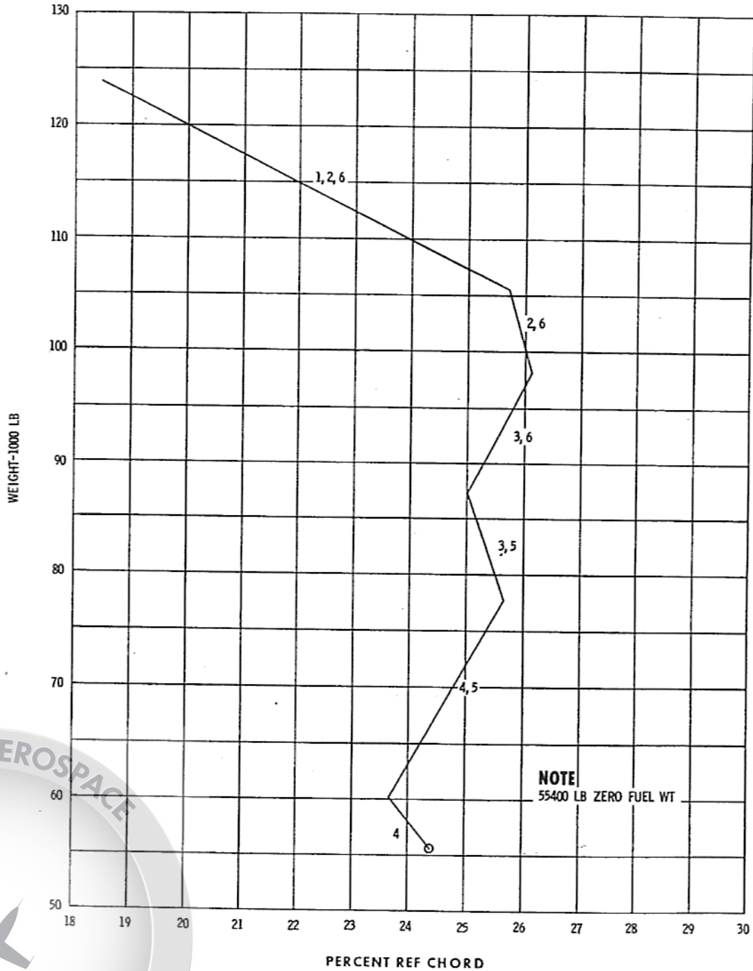
TYPICAL C. G. TRAVEL 6000 LB AFT TRANSFER STOP
