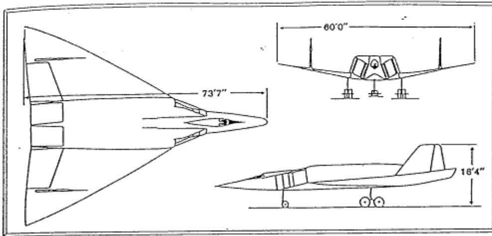
Convair KINGFISH
