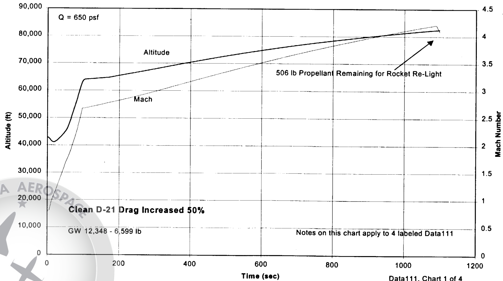
D-21 DRONE with DRACO PROPOSED RBCC ENGINE Fuel - JP-5/LOX, Engine data 16 Sep 99
