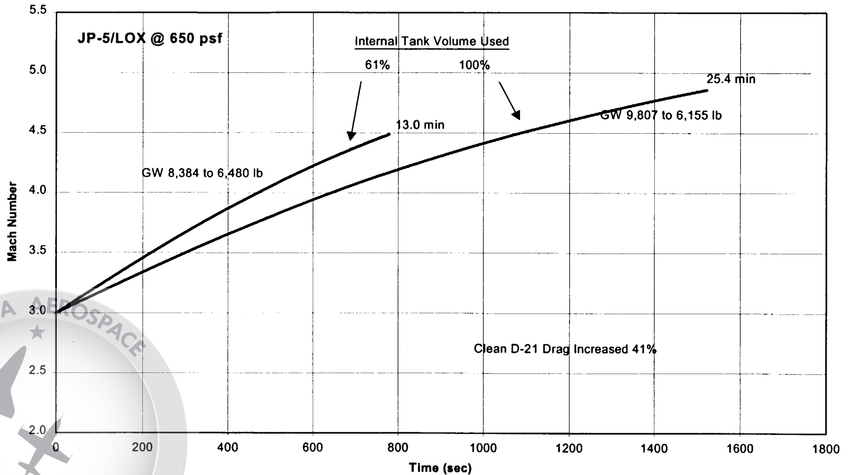
D-21 DRONE with DRACO PROPOSED RBCC ENGINE Comparison of Ramjet Acceleration
