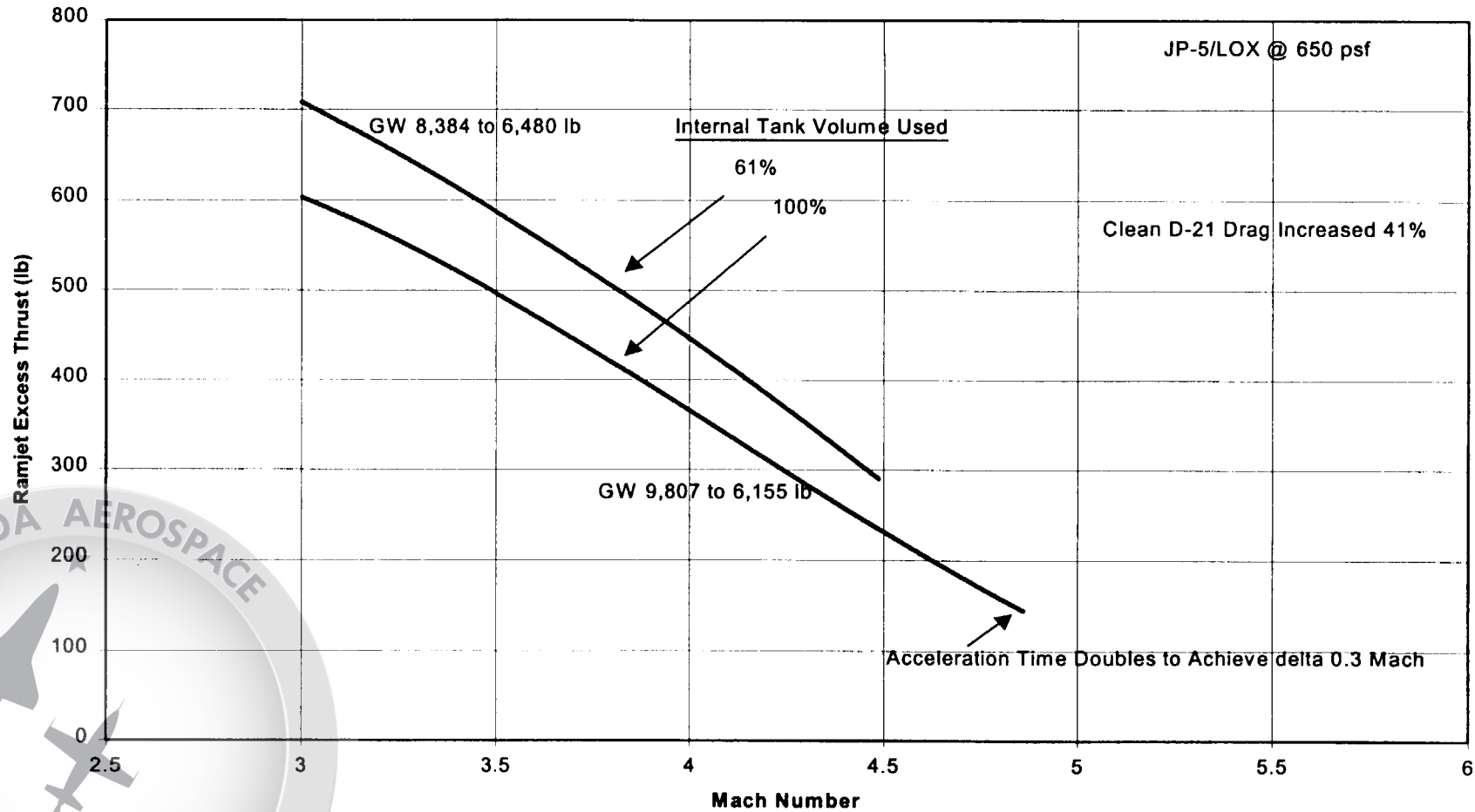
D-21 DRONE with DRACO PROPOSED RBCC ENGINE Comparison of Ramjet Excess Thrust
