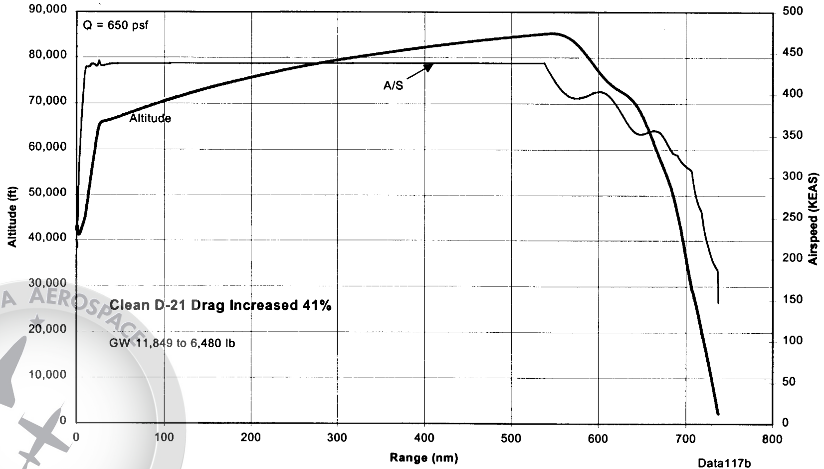
D-21 DRONE with DRACO PROPOSED RBCC ENGINE Fuel - JP-5/LOX, Engine data 16 Sep 99
