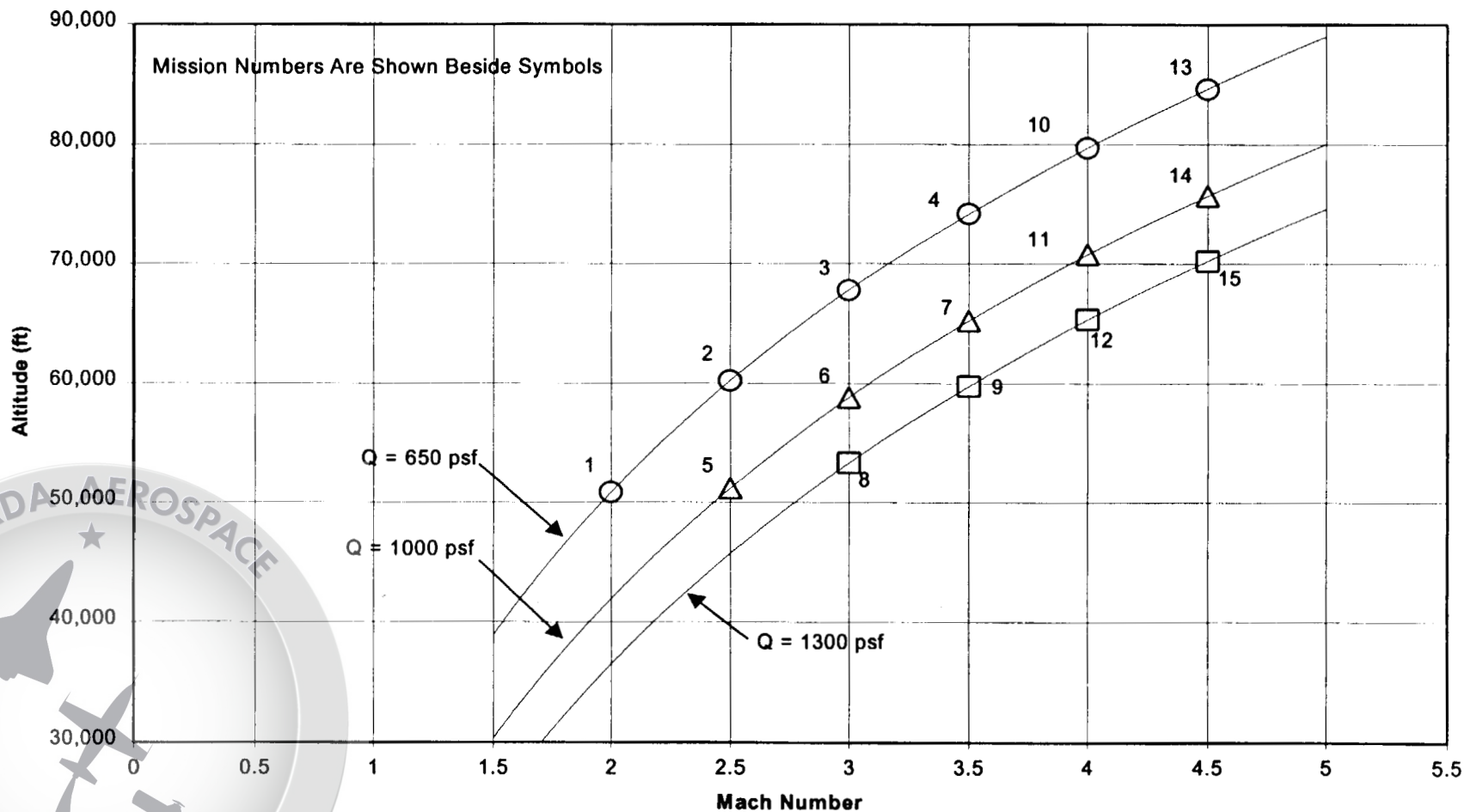
D-21 DRONE with DRACO PROPOSED RBCC ENGINE Envelope Expansion Plan
