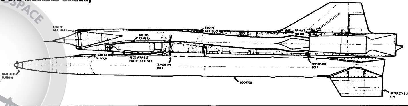
D-21B w/Booster Cutaway
