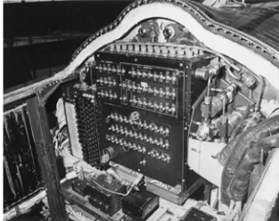
Equipment Bay_2.jpg
