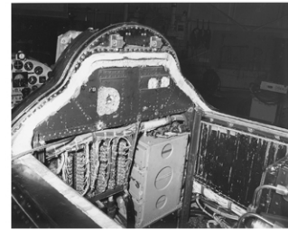
Equipment Bay_1.jpg
